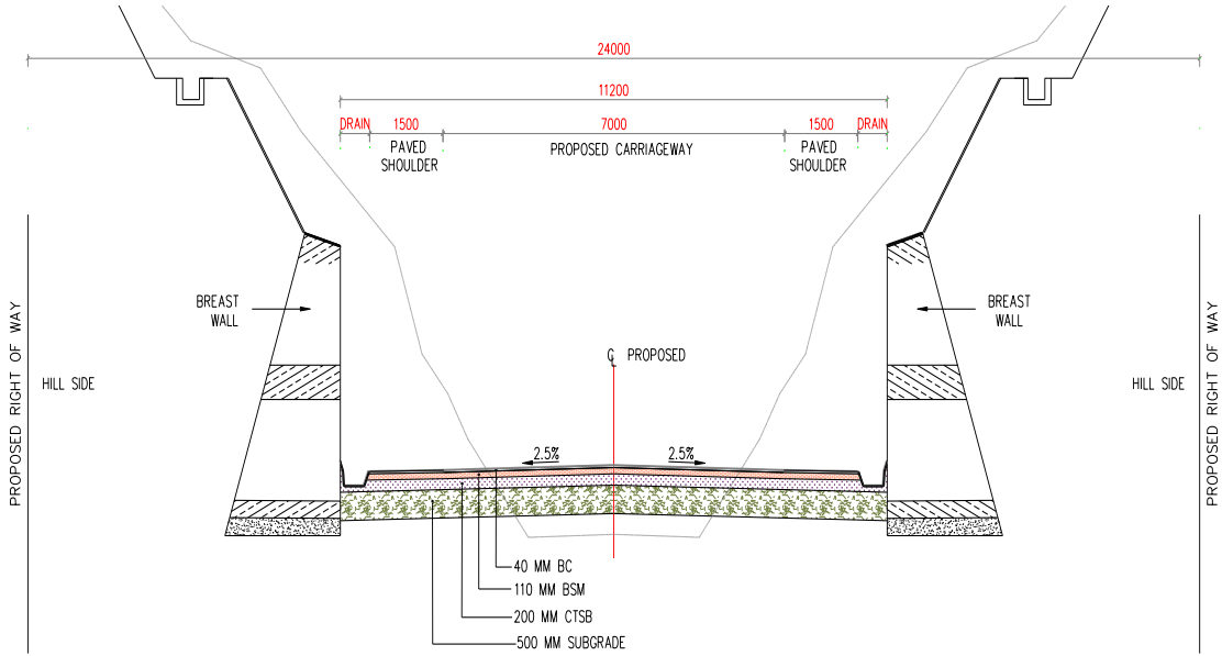
TCS-V Two Lane With Paved Shoulder Raised Portion(Both Side Hill Section)
