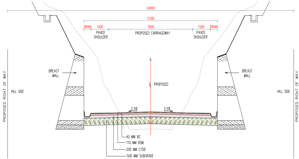
TCS-VIII Two Lane With Paved Shoulder Realignment (Both Side Hill Section)
